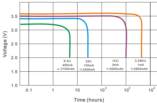
Discharge Characteristics at 23±2°C
