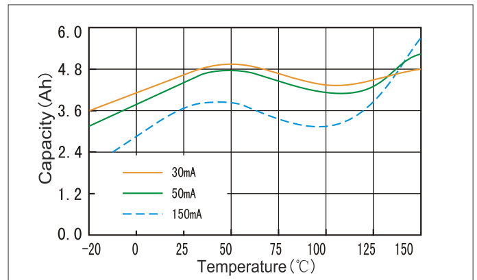
Capacity vs Temperature curve(cut off with 2.0V)
