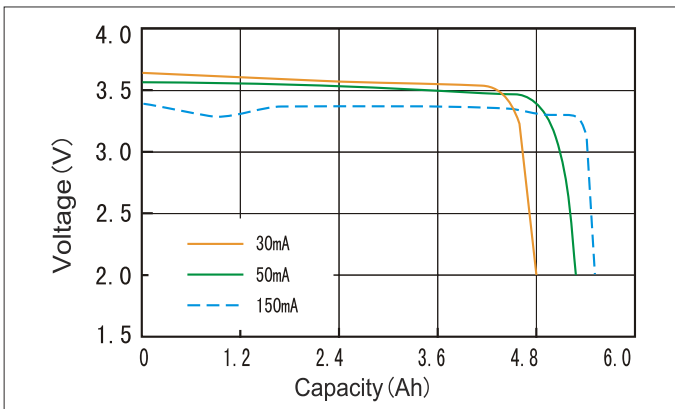
Discharge characteristics at 150°C
