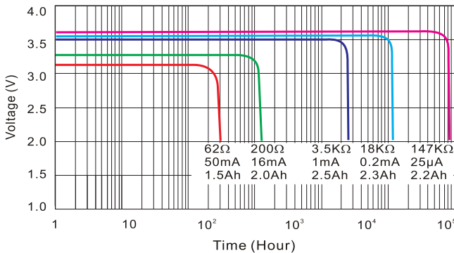
Typical Discharge Profile At 25°C
