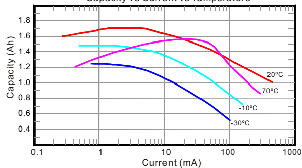
Capacity vs Current vs Temperature
