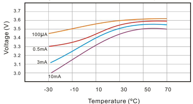
Voltage Plateau Versus Current and Temperature
