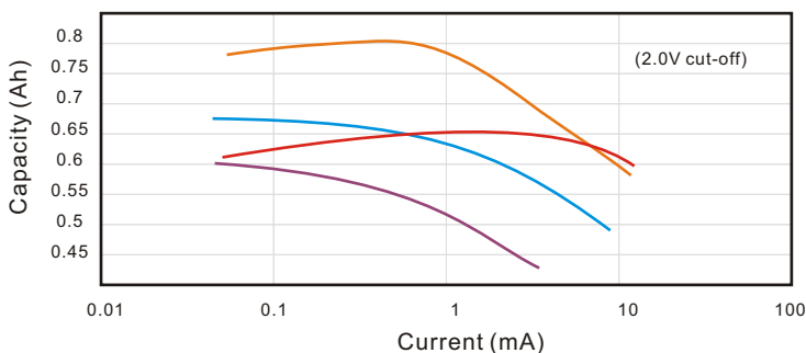
Restored Capacity Versus Current and Temperature
