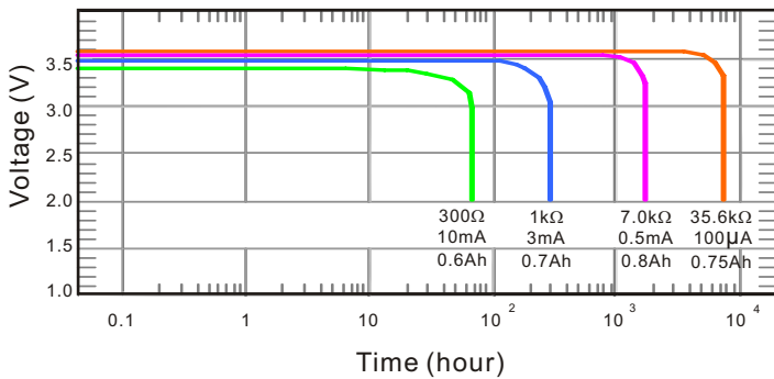
Discharge Characteristics at 23±2°C
