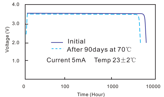
Storage Characteristics
