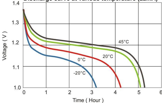
Discharge curve at various temperature (22mA)
