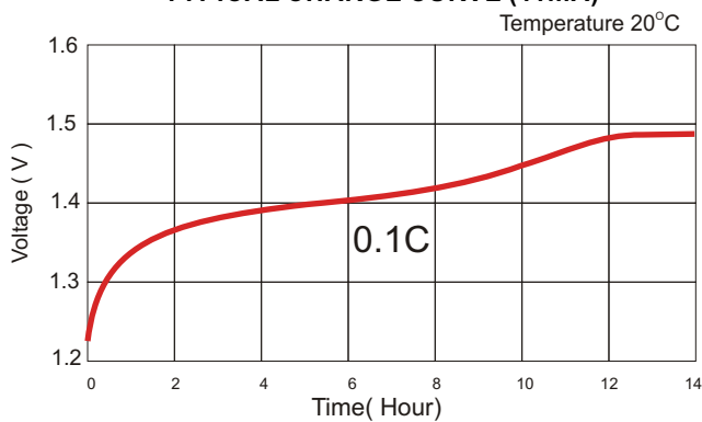
TYPICAL CHARGE CURVE (11mA)
