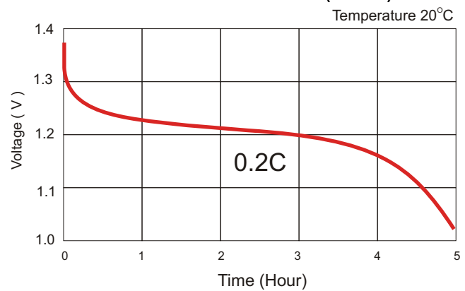
TYPICAL DISCHARGE CURVE (3.6mA)
