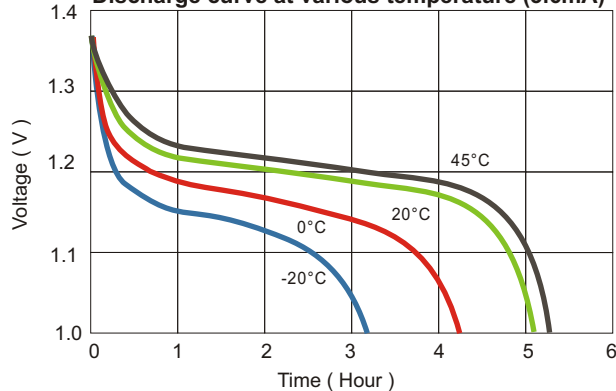
Discharge curve at various temperature (3.6mA)
