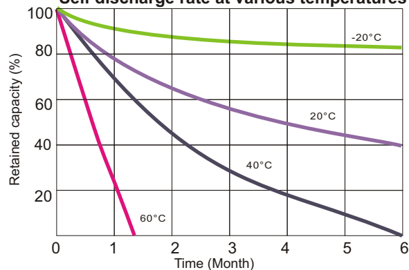
Self discharge rate at various temperatures
