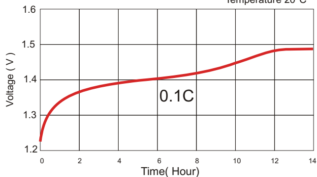
TYPICAL CHARGE CURVE (1.8mA)
