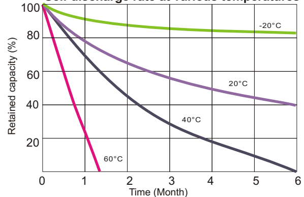
Self discharge rate at various temperatures
