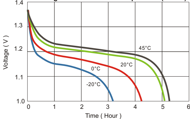
Discharge curve at various temperature (3.6mA)
