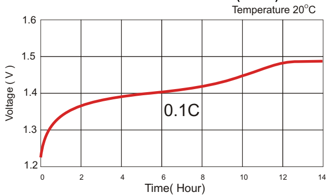
TYPICAL CHARGE CURVE (23mA)
