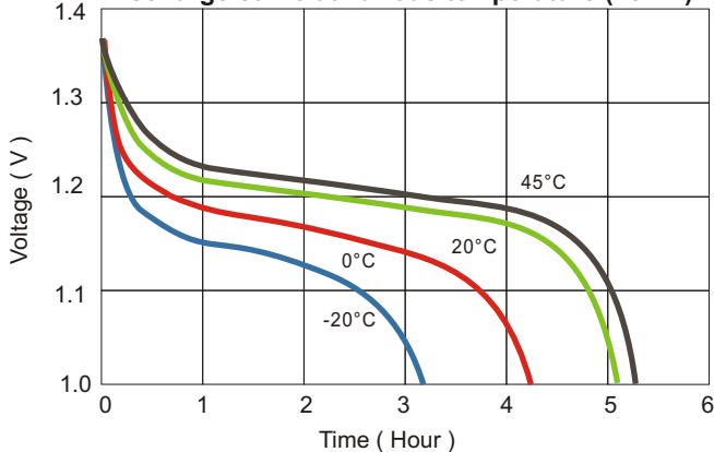
Discharge curve at various temperature (46mA)
