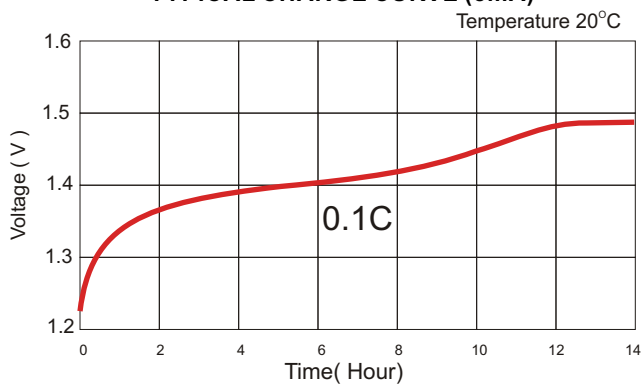
TYPICAL CHARGE CURVE (8mA)
