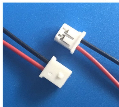
MOLEX510040200
