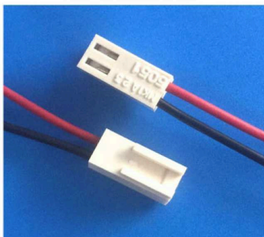
MOLEX5051-2P
