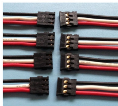
MOLEX781720300
