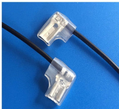
187 Flag type terminal wires
