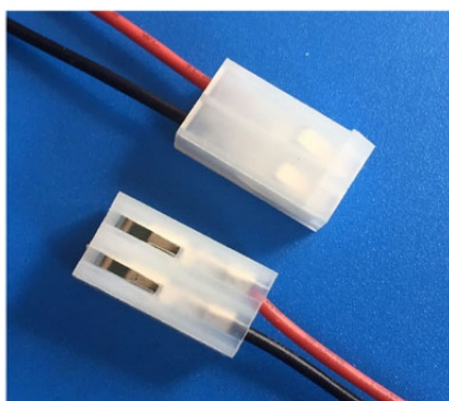
MOLEX2139-2P
