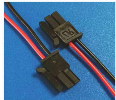
MOLEX430250200
