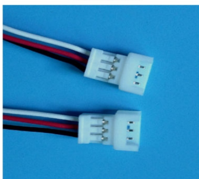
MOLEX510470300
