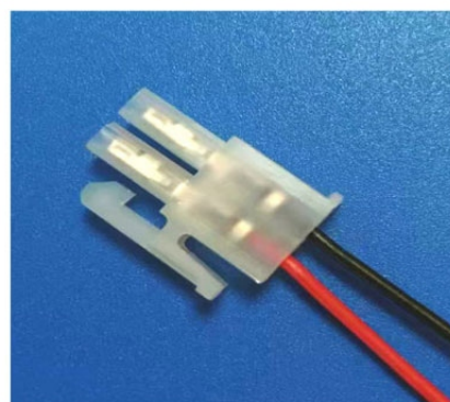
MOLEX5557-2P(1*2)
